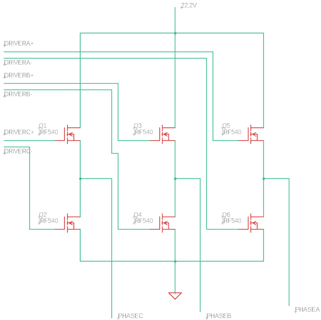
Figure 19: Mosfet Schematic
