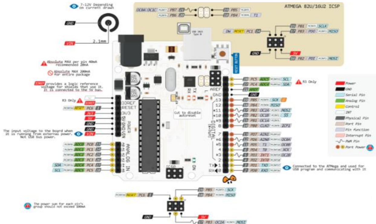
Figure 6: Arduino Uno Pins
