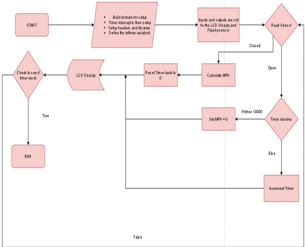
Figure 22: Flipsky Sensor Calculation Flow Chart
