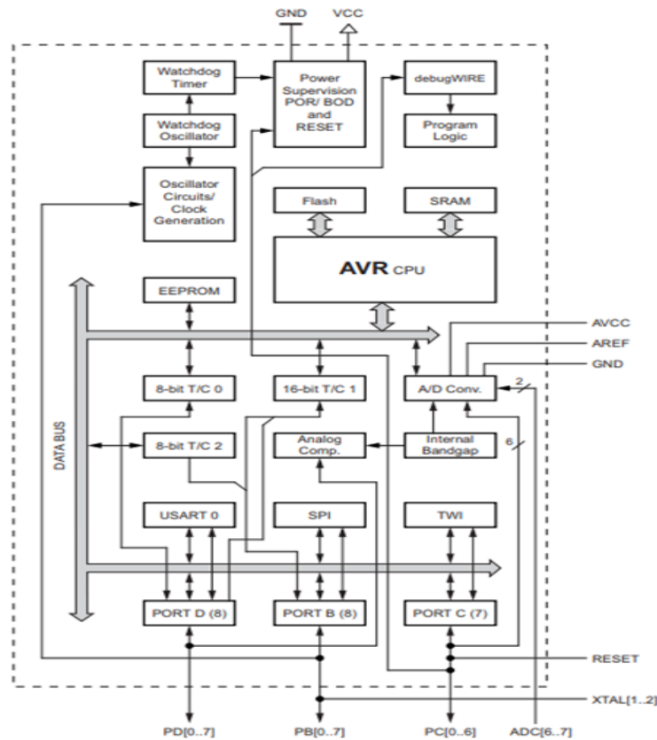
Arduino Uno Rev3 Block Diagram
