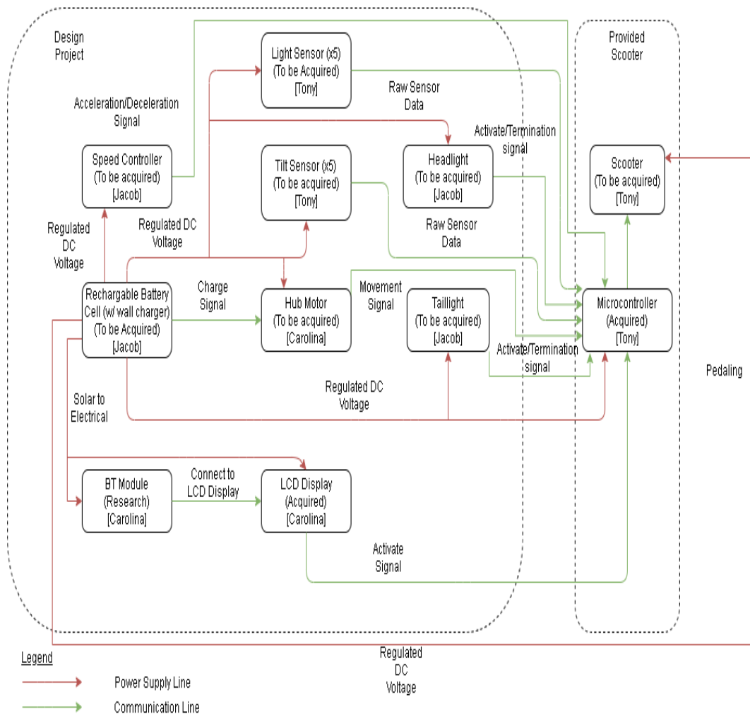
Figure 21: Hardware design
