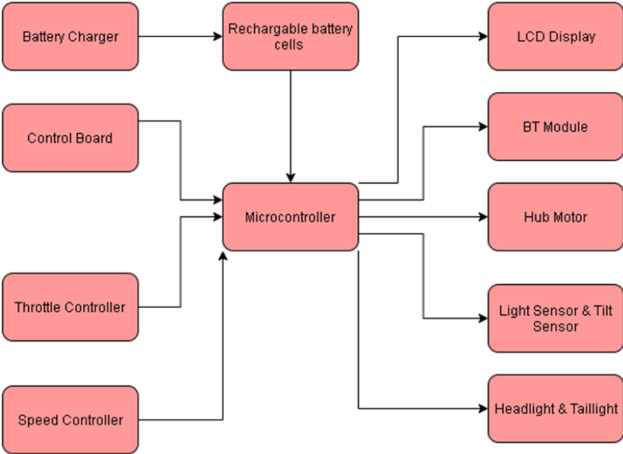
Figure 9: Top Level System
